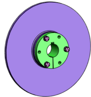
TUSA Doc – (T-1001) Sure-Grip Bushing & Rotor Assembly (Taper lock with disc, QD)
