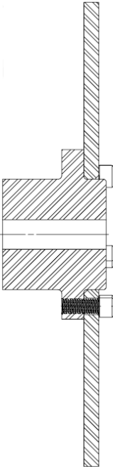
TUSA Doc – (T-1004) Disc and Hub Assembly
