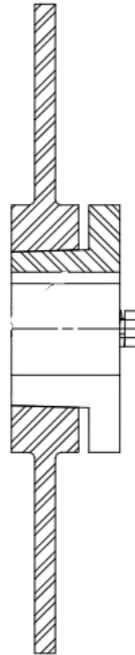
TUSA Doc – (T-1001) Sure-Grip Bushing & Rotor Assembly (Taper lock with disc, QD)
