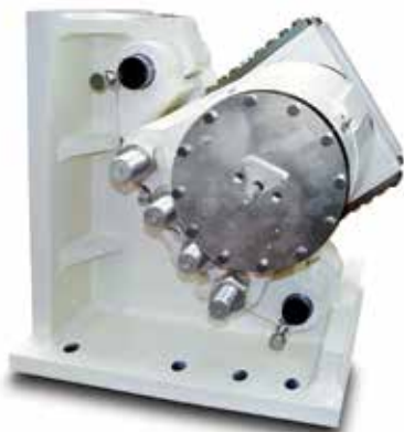
The VMS-FL has a braking force rating of 460 kN which assumes a coefficient of friction of 0.4 and 2 mm pad air gap.
